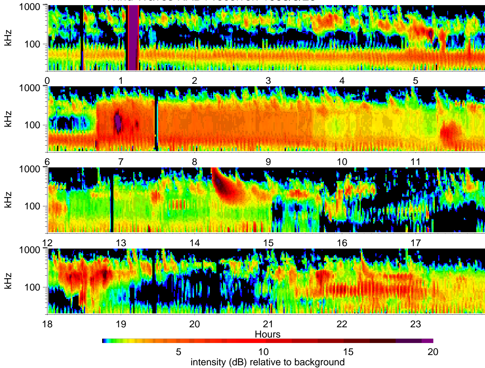
Wind Waves RAD1 receiver: 1998/8/26
