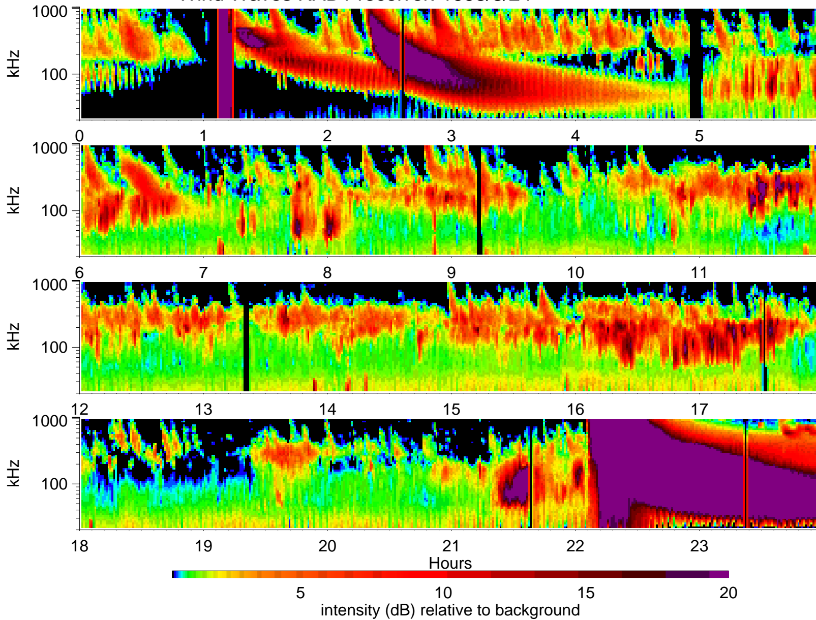
Wind Waves RAD1 receiver: 1998/8/24
