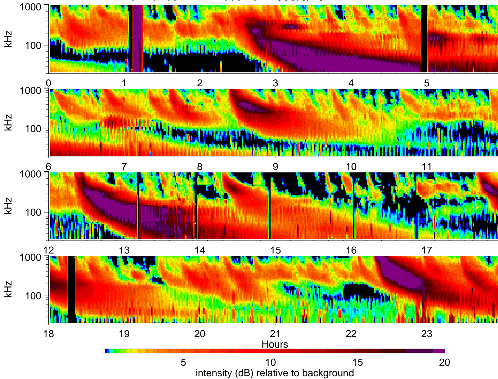
Wind Waves RAD1 receiver: 1998/8/18
