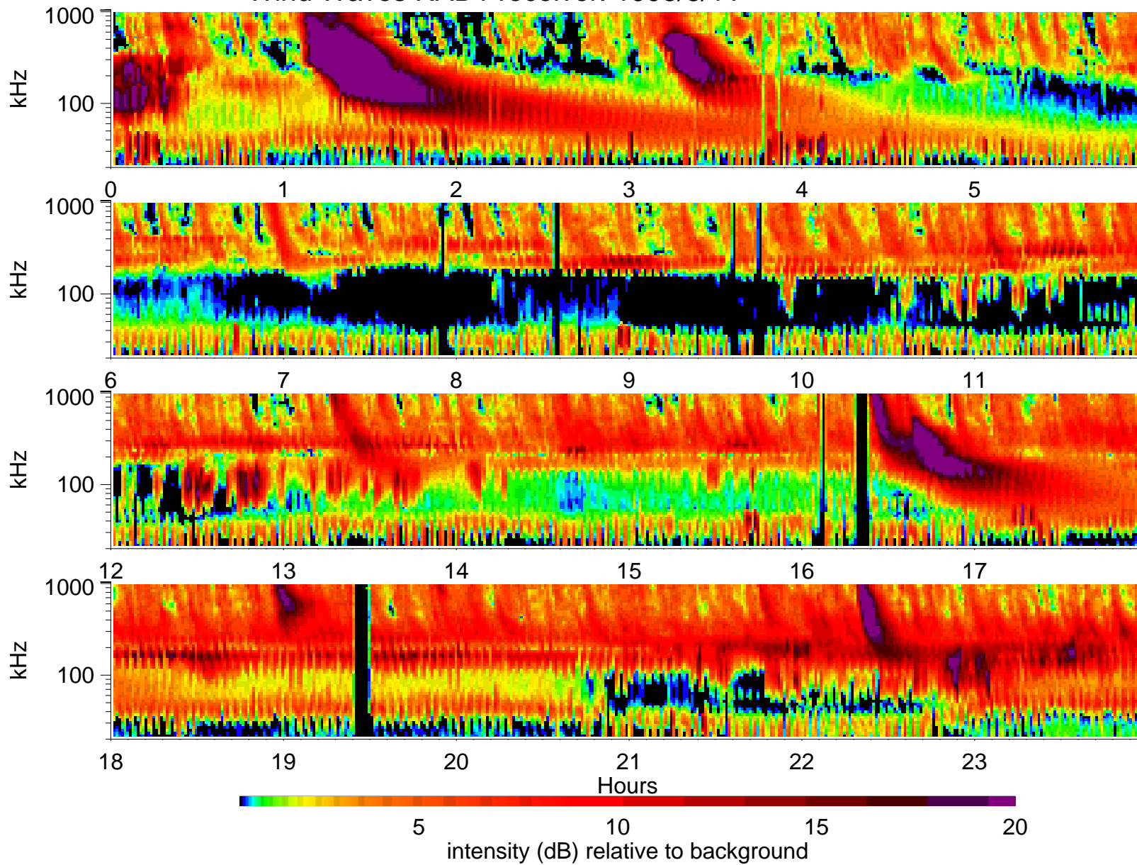
Wind Waves RAD1 receiver: 1998/8/11
