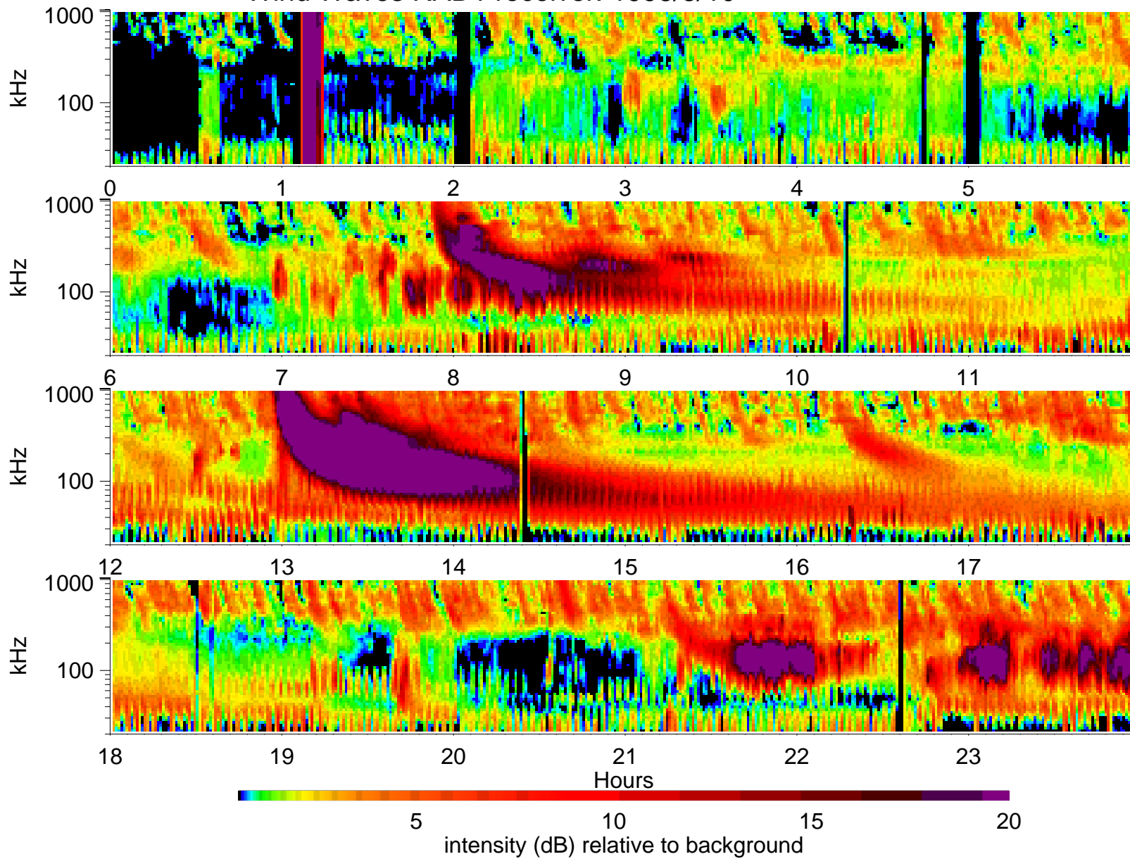
Wind Waves RAD1 receiver: 1998/8/10
