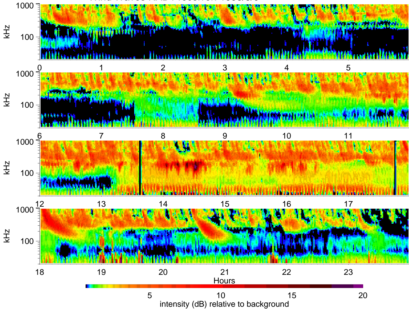
Wind Waves RAD1 receiver: 1998/8/9
