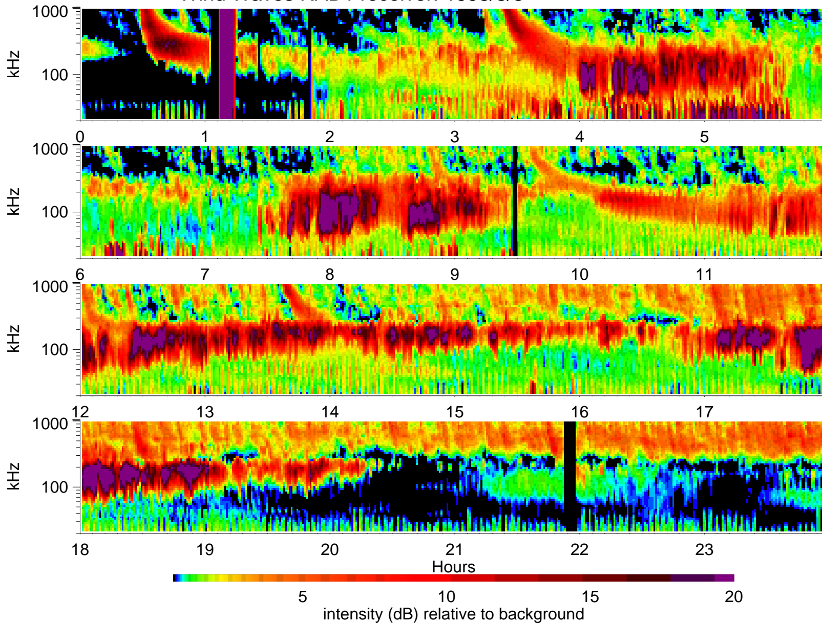
Wind Waves RAD1 receiver: 1998/8/8
