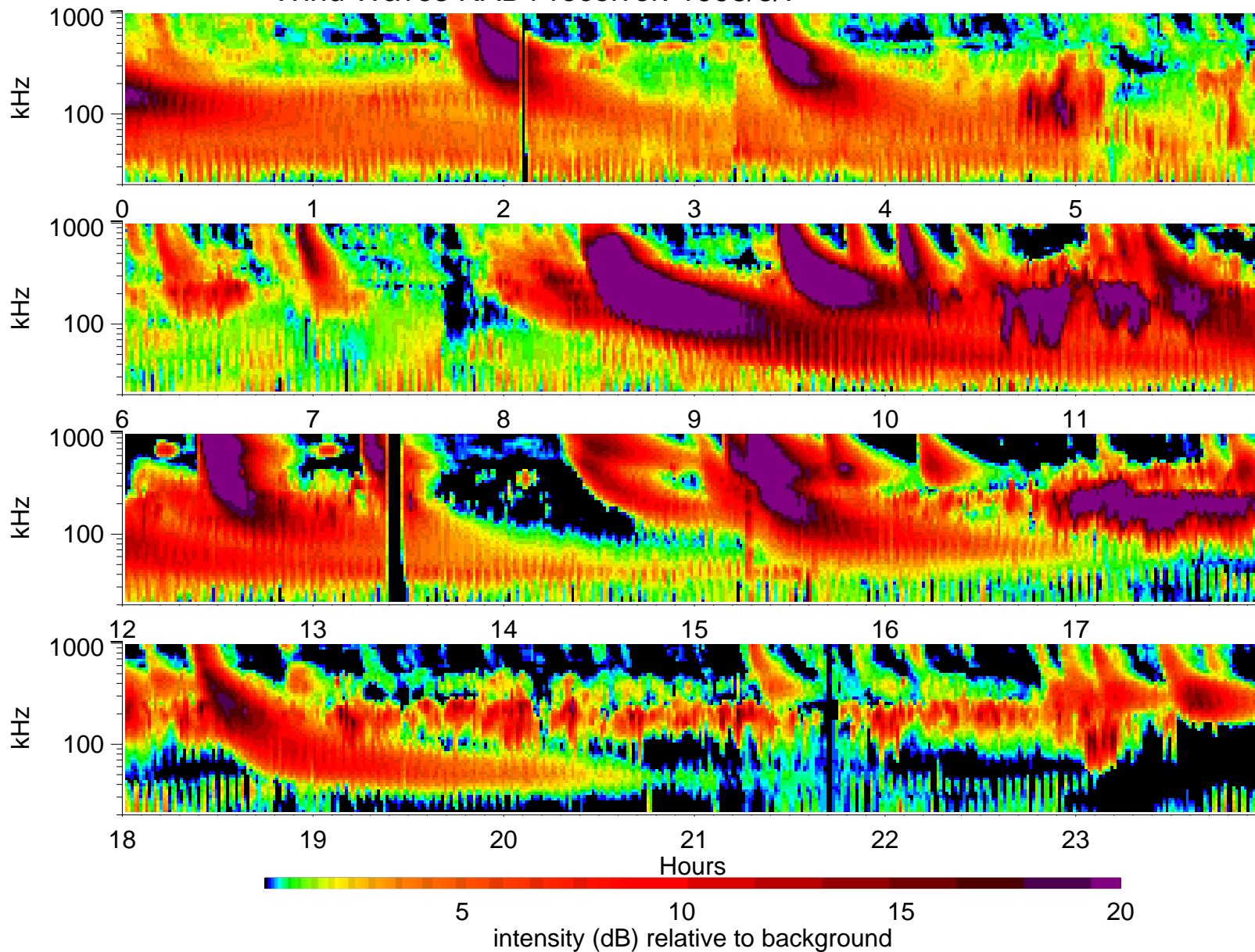
Wind Waves RAD1 receiver: 1998/8/7
