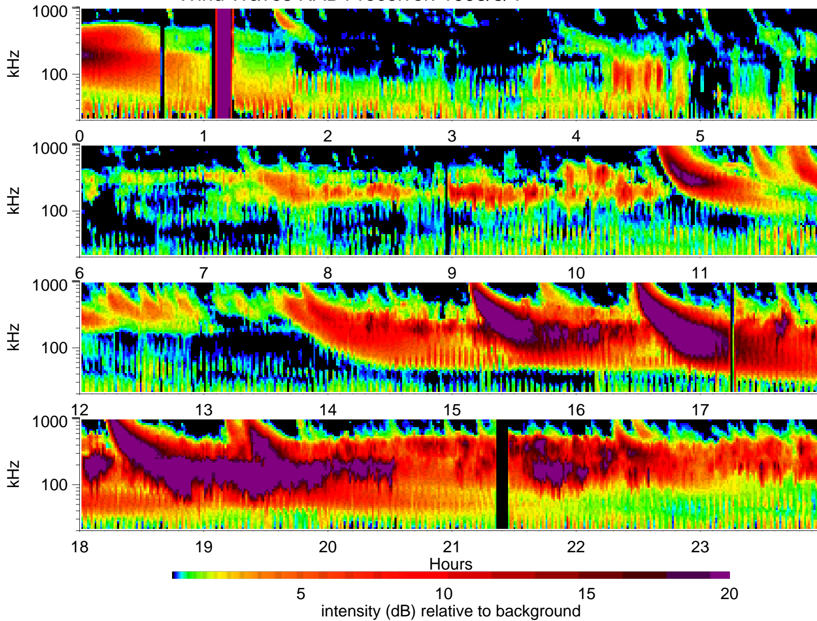
Wind Waves RAD1 receiver: 1998/8/4
