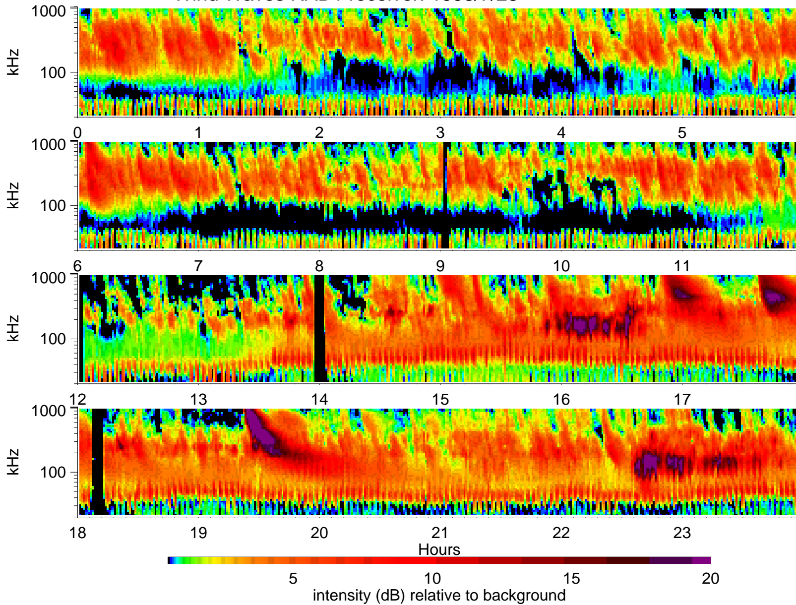
Wind Waves RAD1 receiver: 1998/7/28
