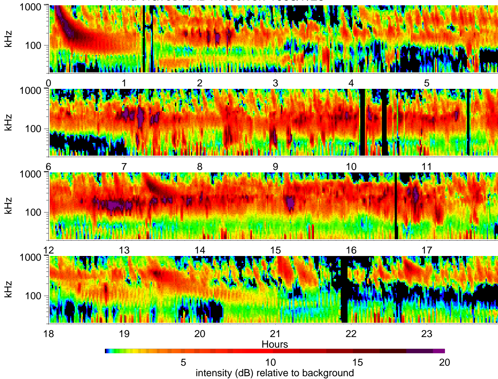
Wind Waves RAD1 receiver: 1998/7/26
