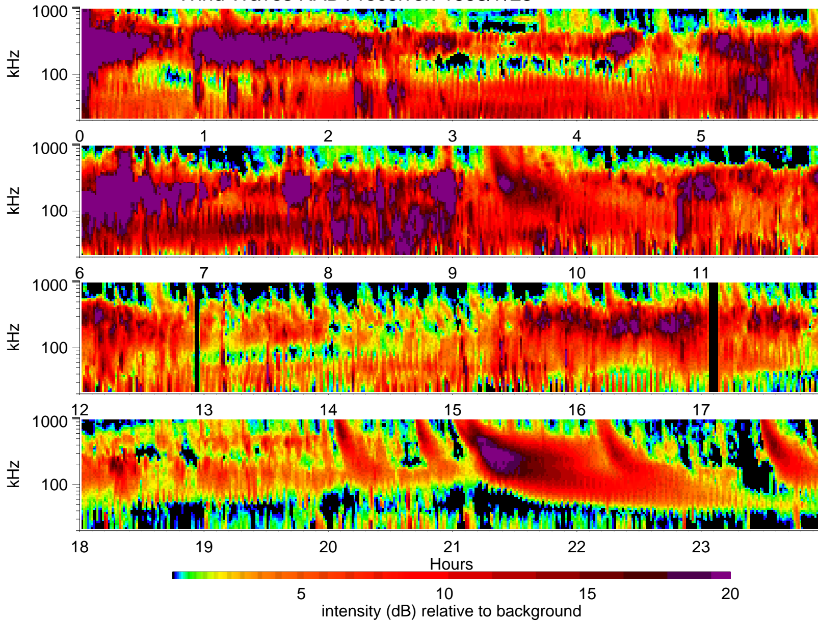
Wind Waves RAD1 receiver: 1998/7/25
