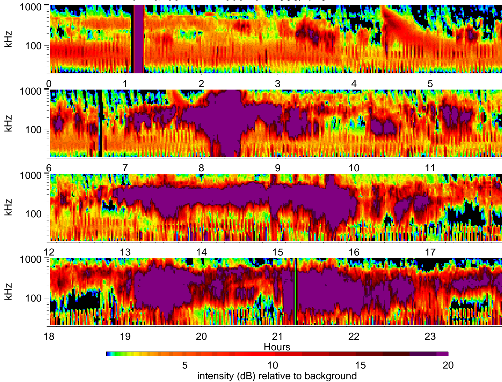
Wind Waves RAD1 receiver: 1998/7/23
