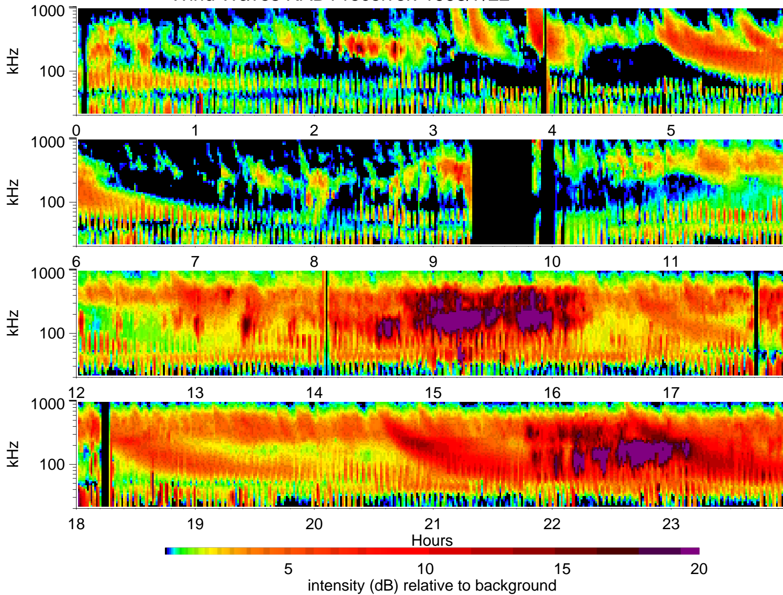
Wind Waves RAD1 receiver: 1998/7/22
