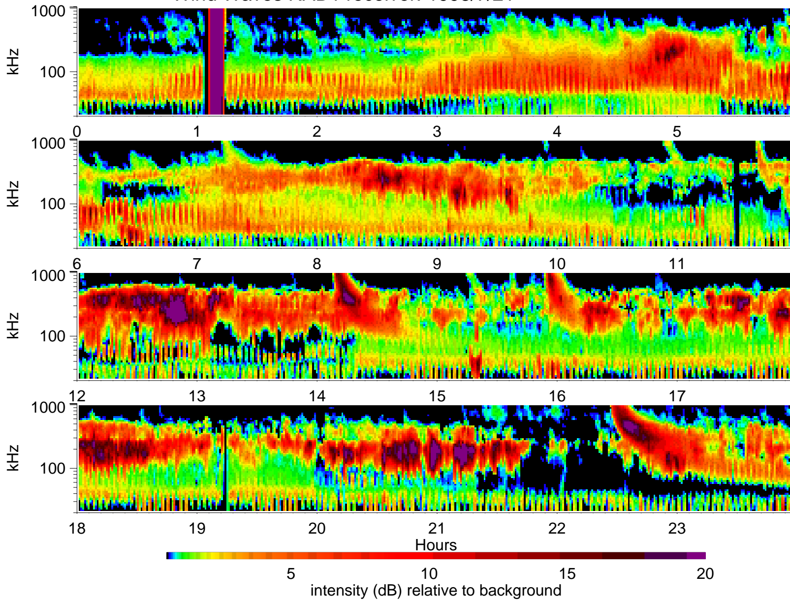
Wind Waves RAD1 receiver: 1998/7/21
