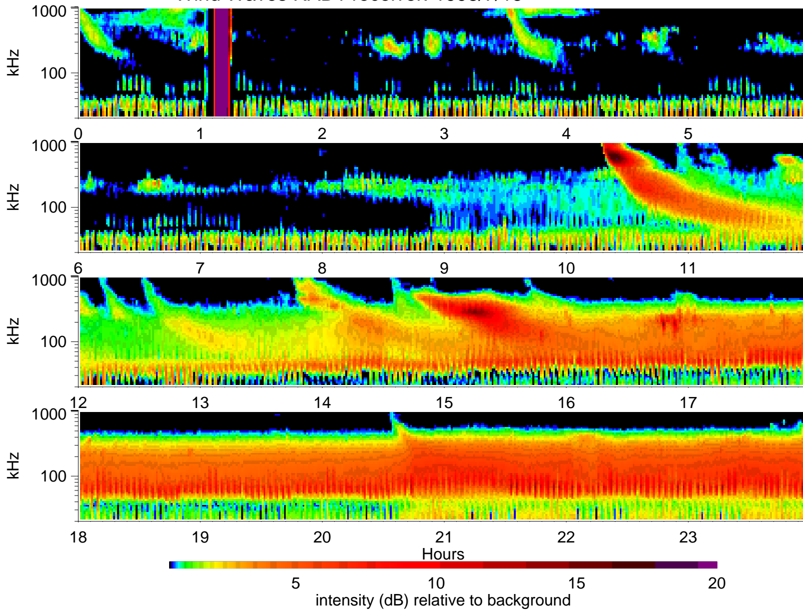
Wind Waves RAD1 receiver: 1998/7/15
