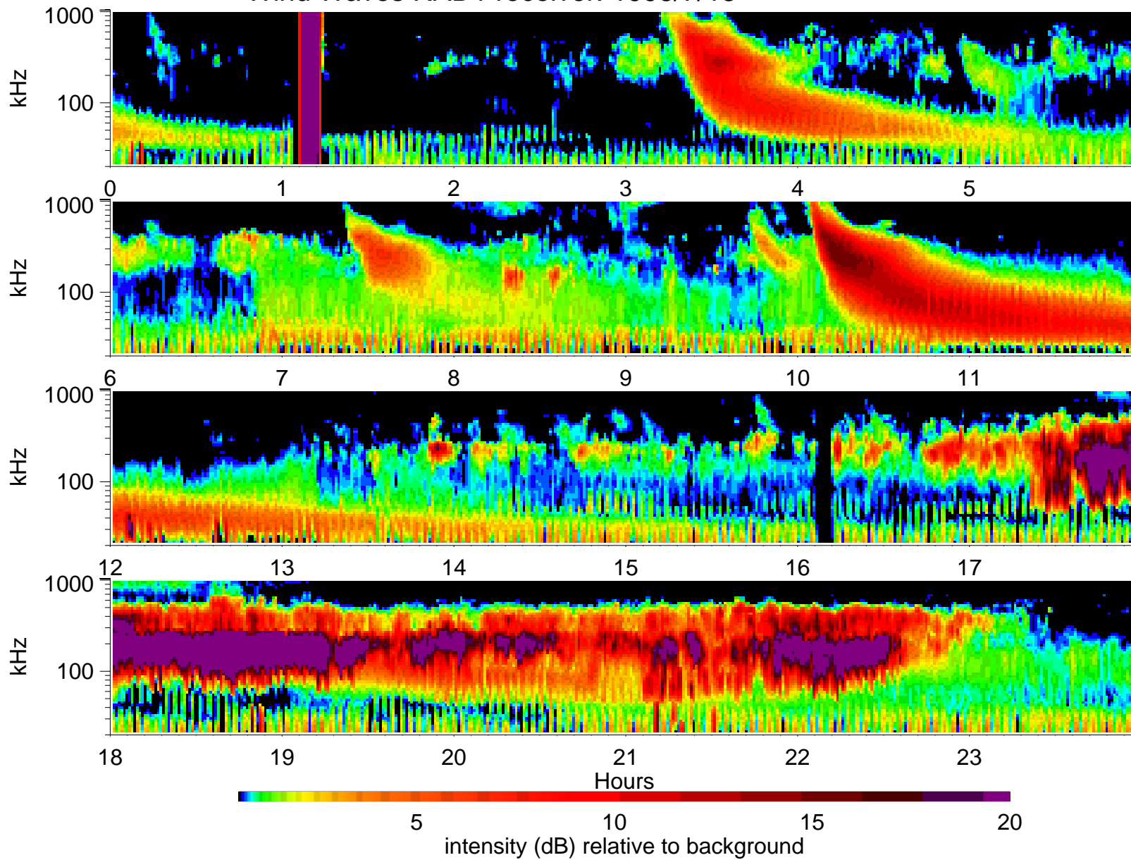
Wind Waves RAD1 receiver: 1998/7/13
