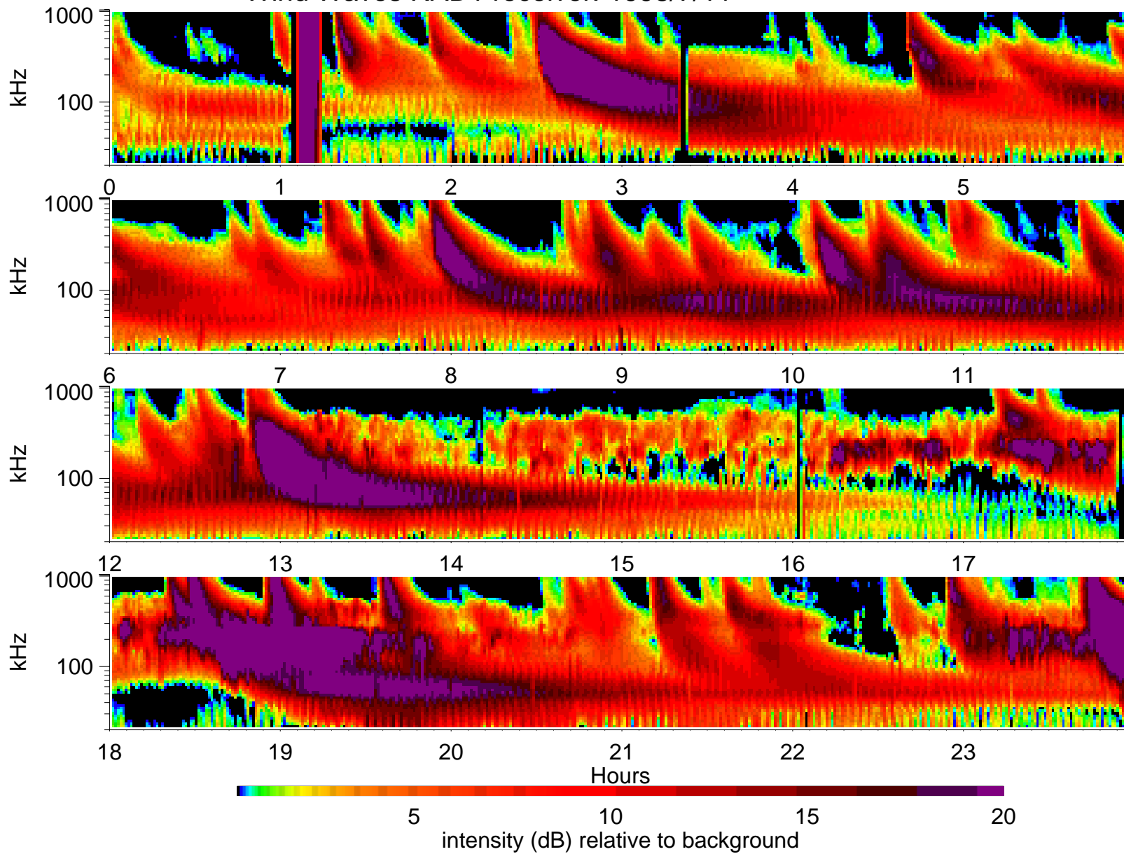
Wind Waves RAD1 receiver: 1998/7/11
