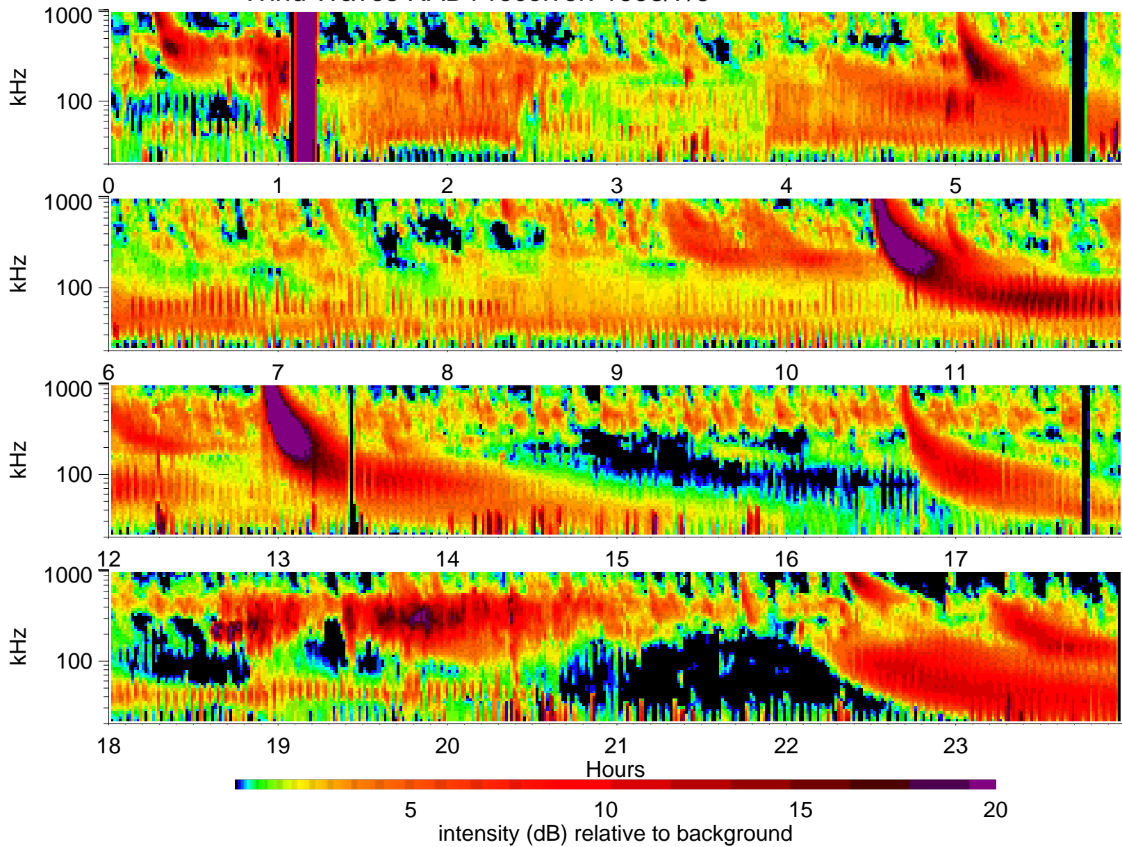
Wind Waves RAD1 receiver: 1998/7/5
