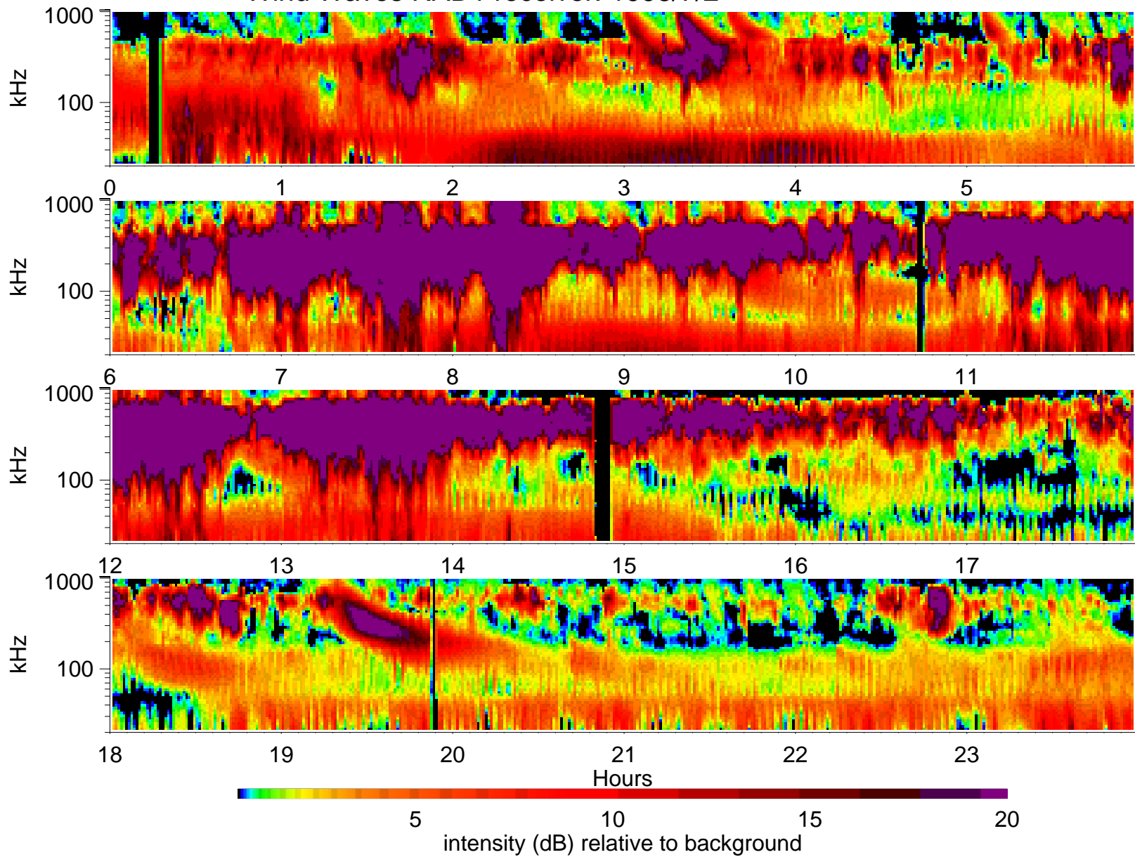
Wind Waves RAD1 receiver: 1998/7/2
