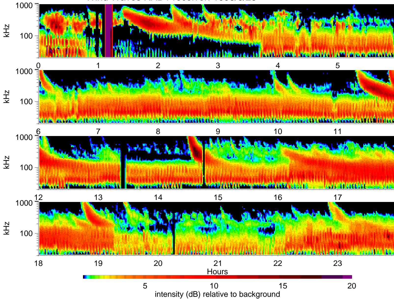
Wind Waves RAD1 receiver: 1998/6/25
