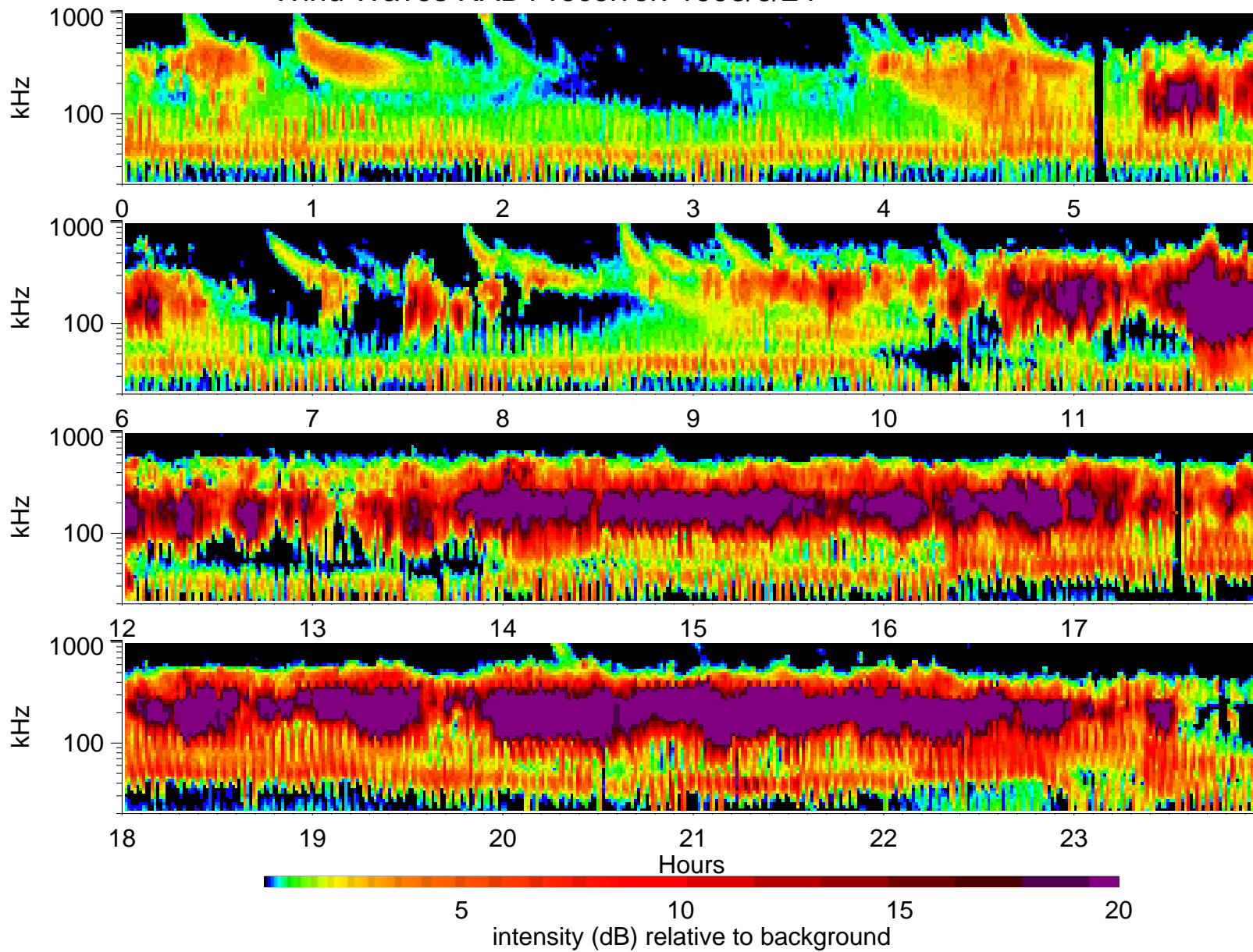
Wind Waves RAD1 receiver: 1998/6/24
