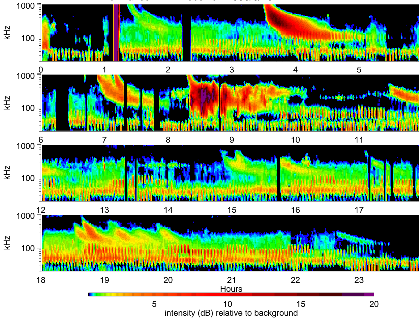
Wind Waves RAD1 receiver: 1998/6/19
