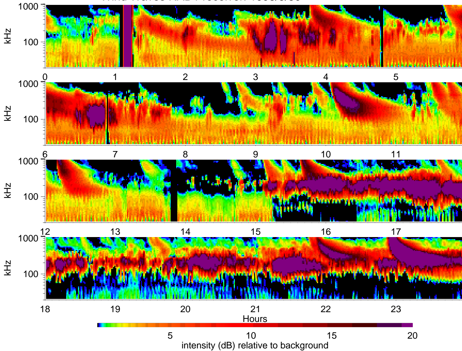
Wind Waves RAD1 receiver: 1998/5/30
