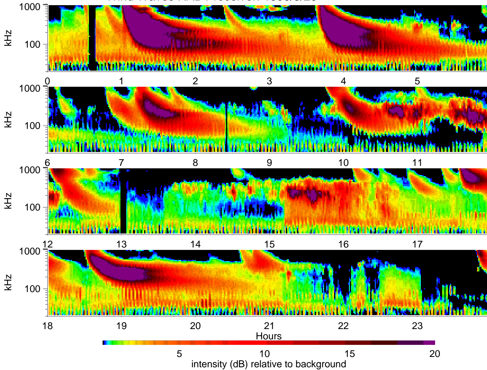
Wind Waves RAD1 receiver: 1998/5/29
