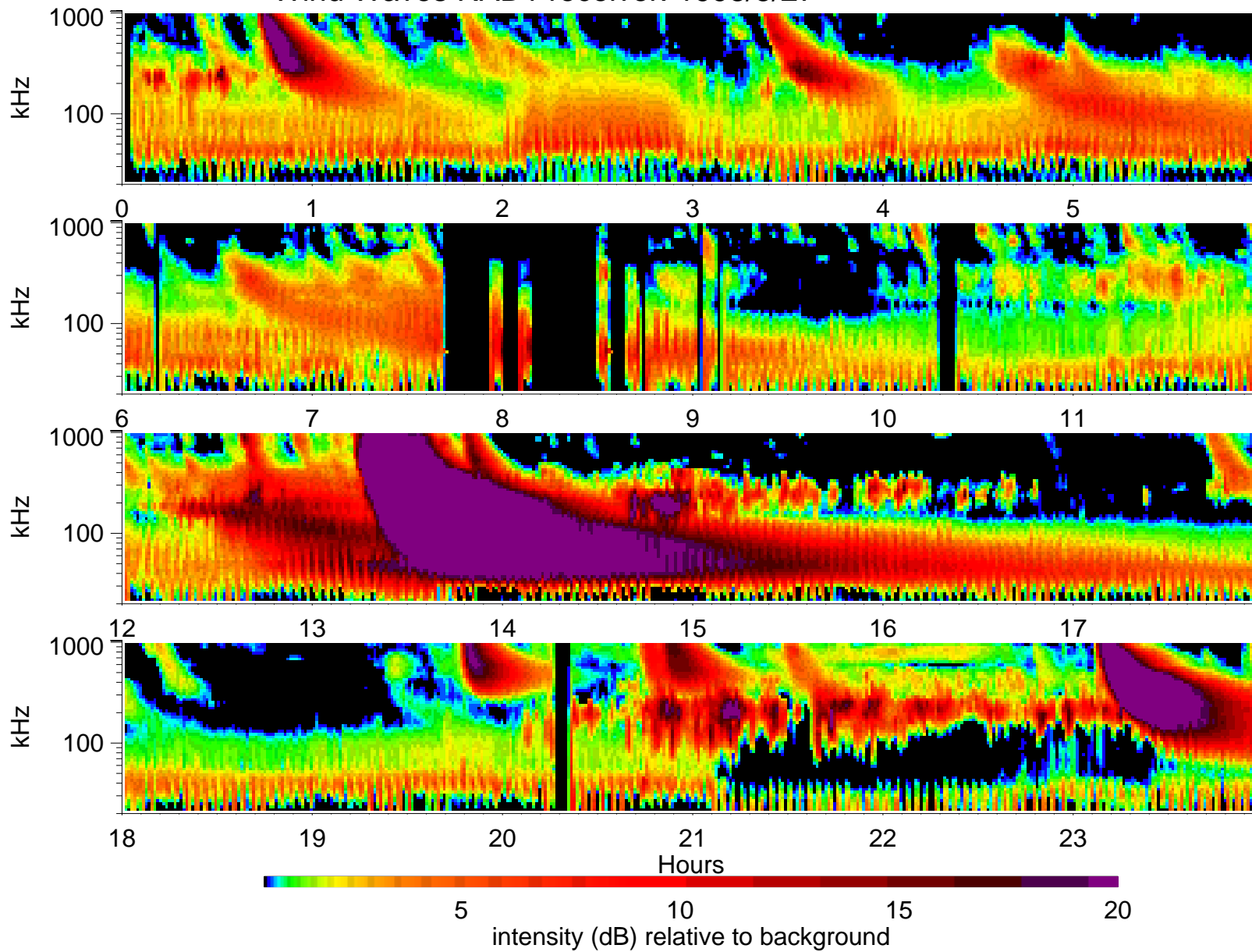
Wind Waves RAD1 receiver: 1998/5/27
