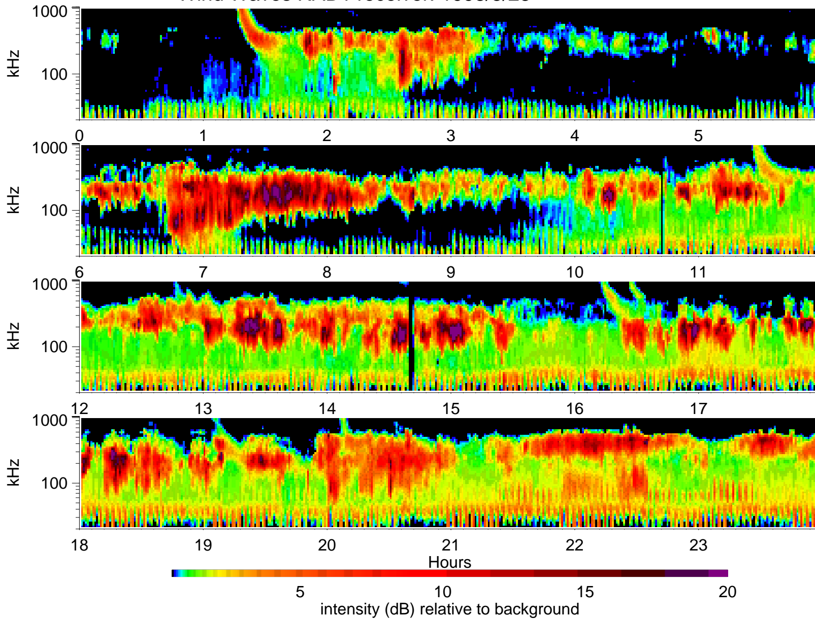
Wind Waves RAD1 receiver: 1998/5/23
