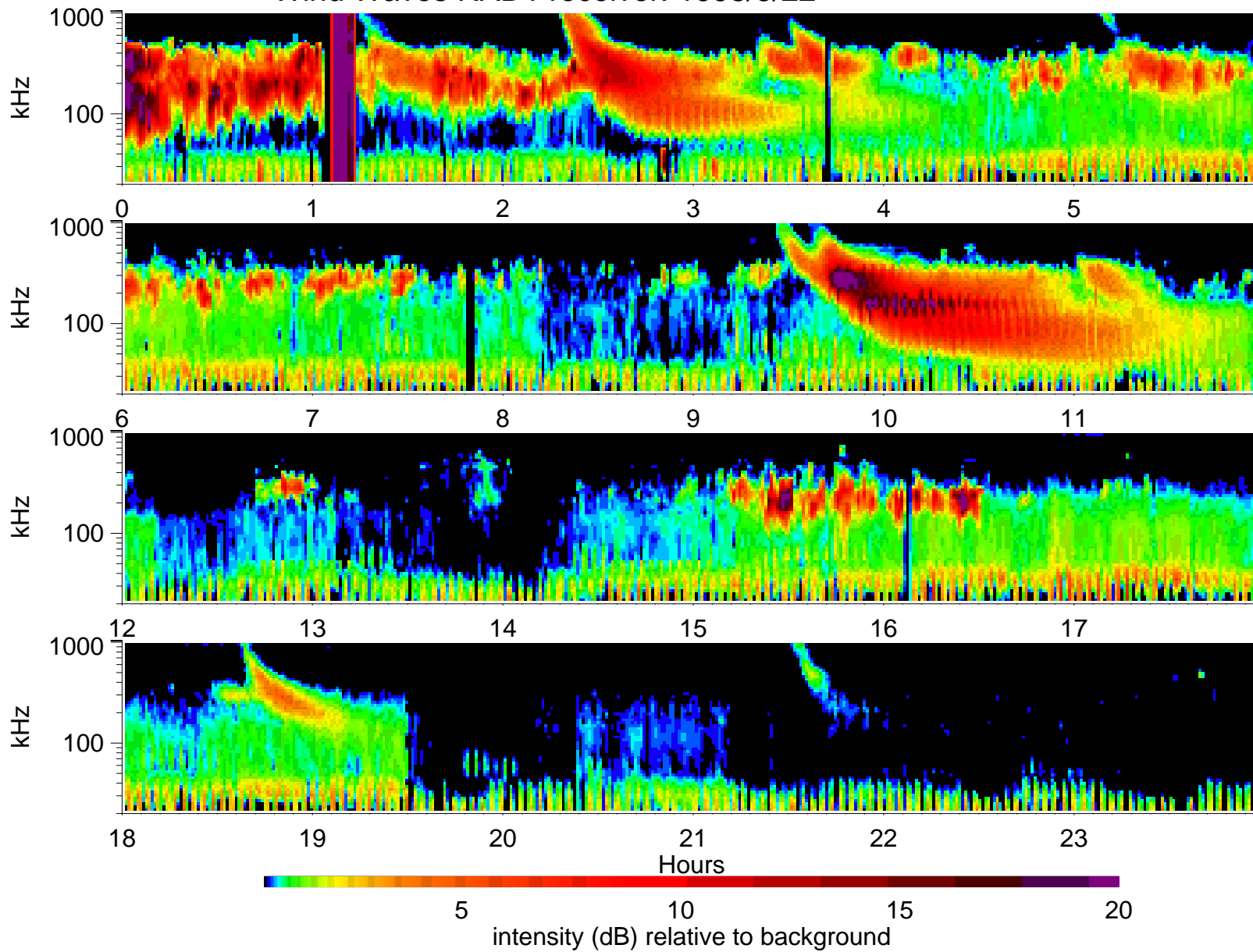
Wind Waves RAD1 receiver: 1998/5/22
