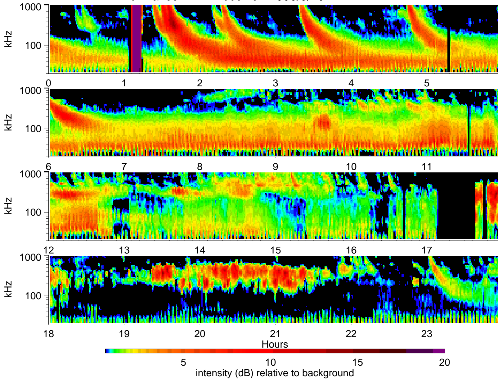
Wind Waves RAD1 receiver: 1998/5/20
