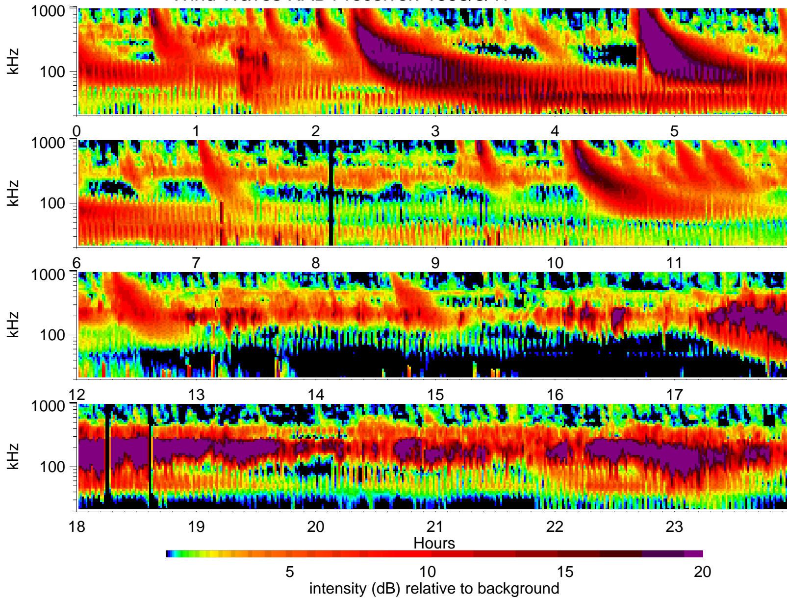
Wind Waves RAD1 receiver: 1998/5/17
