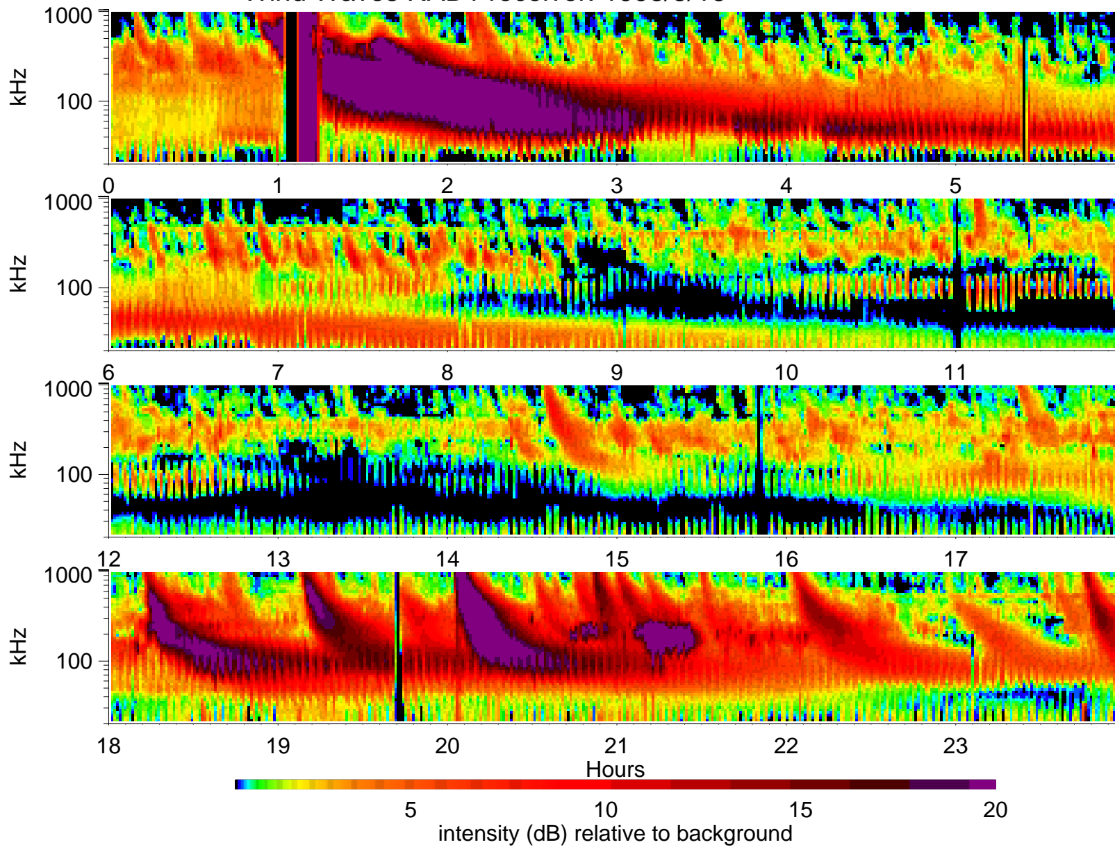
Wind Waves RAD1 receiver: 1998/5/16
