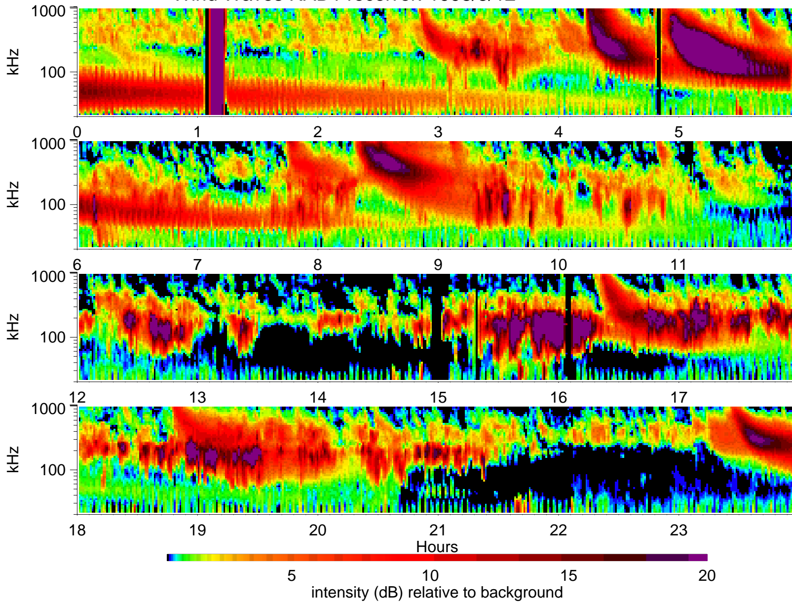
Wind Waves RAD1 receiver: 1998/5/12
