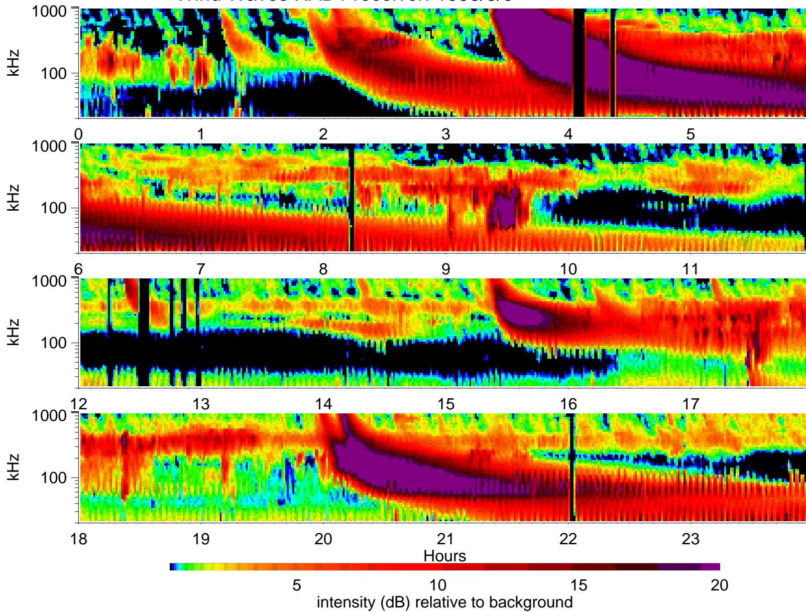
Wind Waves RAD1 receiver: 1998/5/9
