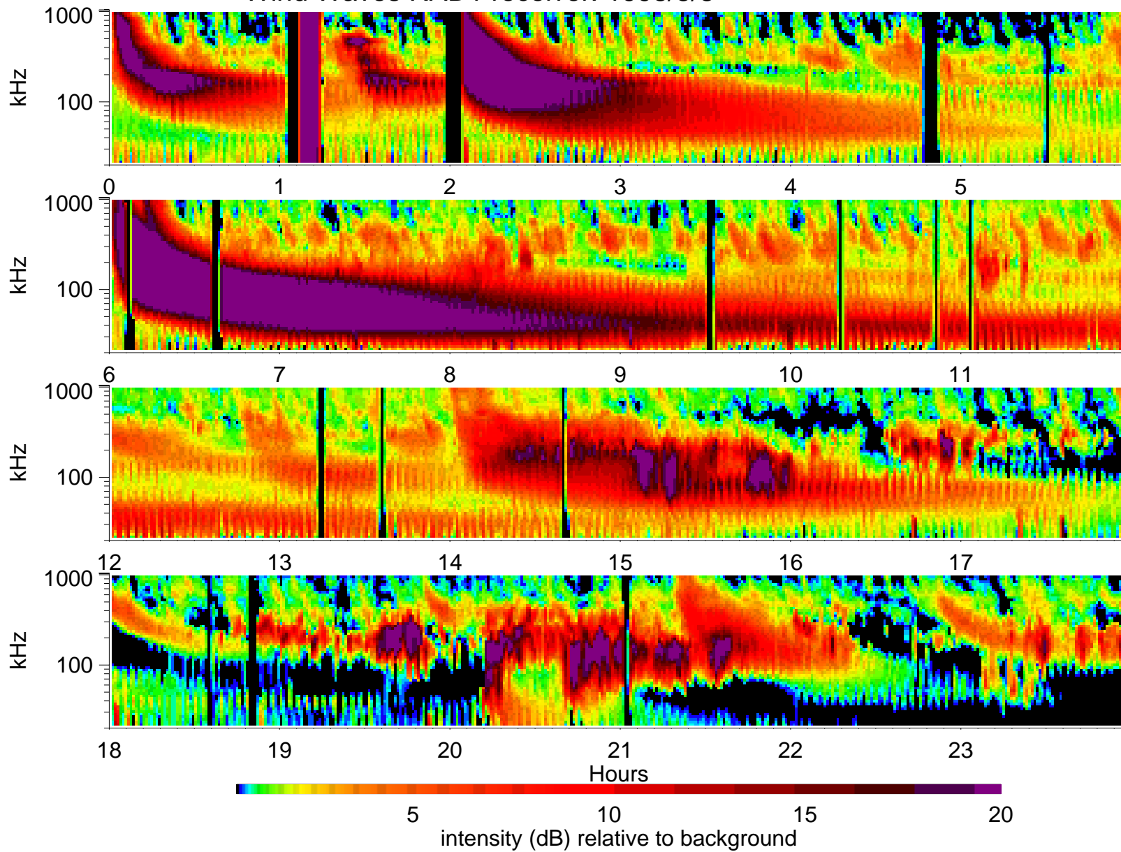
Wind Waves RAD1 receiver: 1998/5/8
