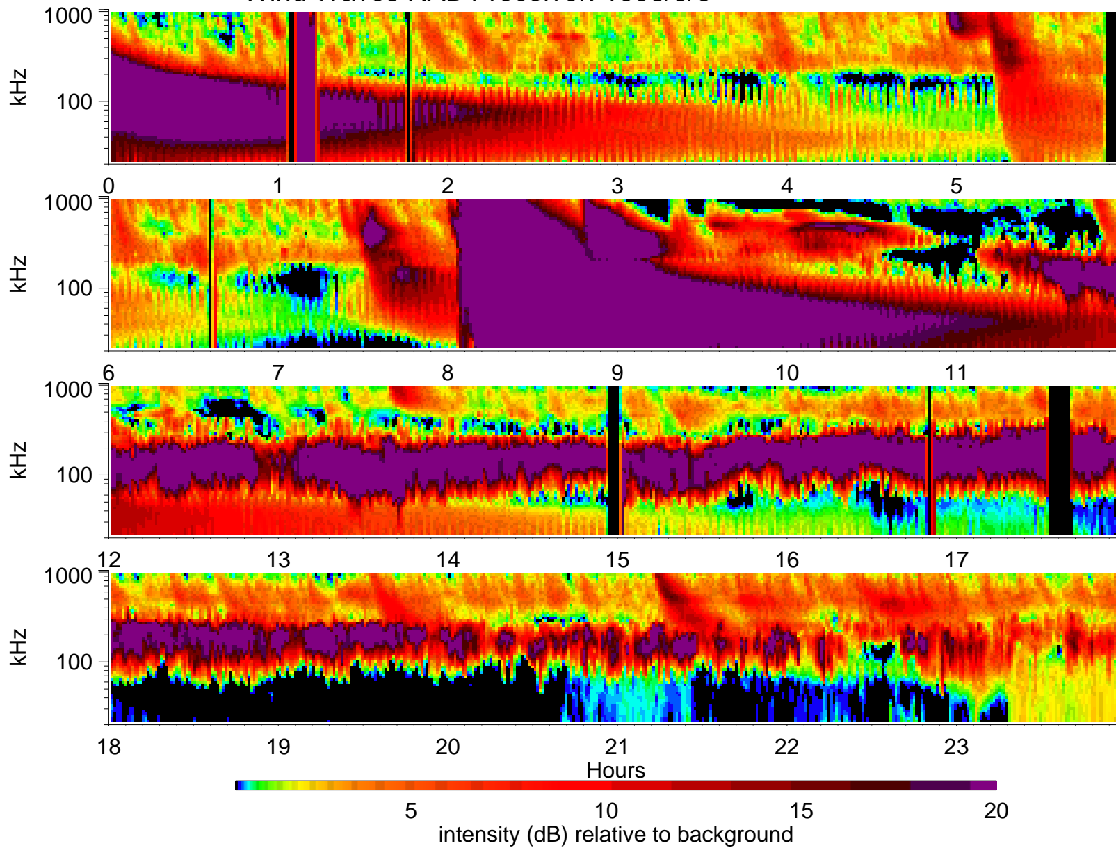
Wind Waves RAD1 receiver: 1998/5/6
