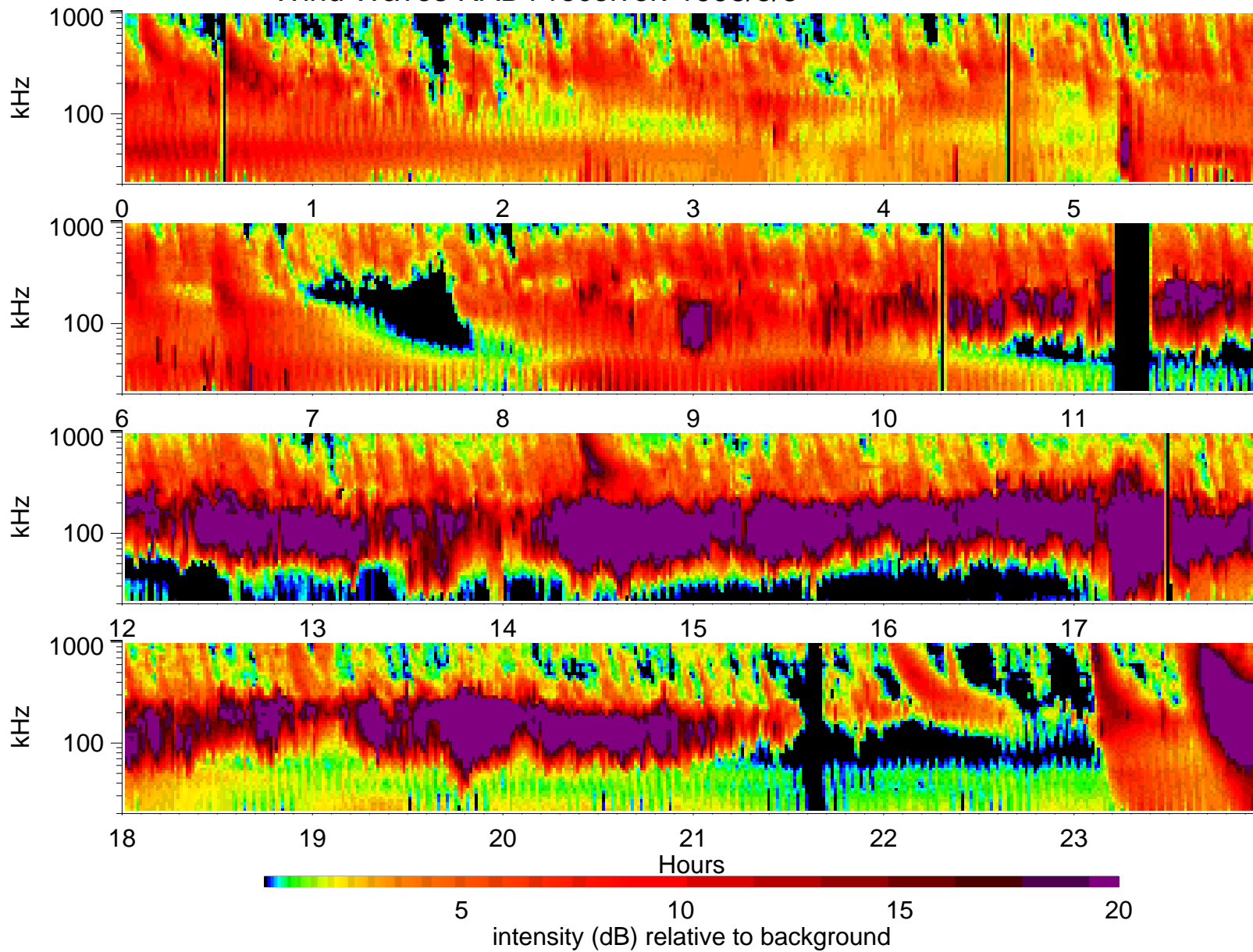
Wind Waves RAD1 receiver: 1998/5/5
