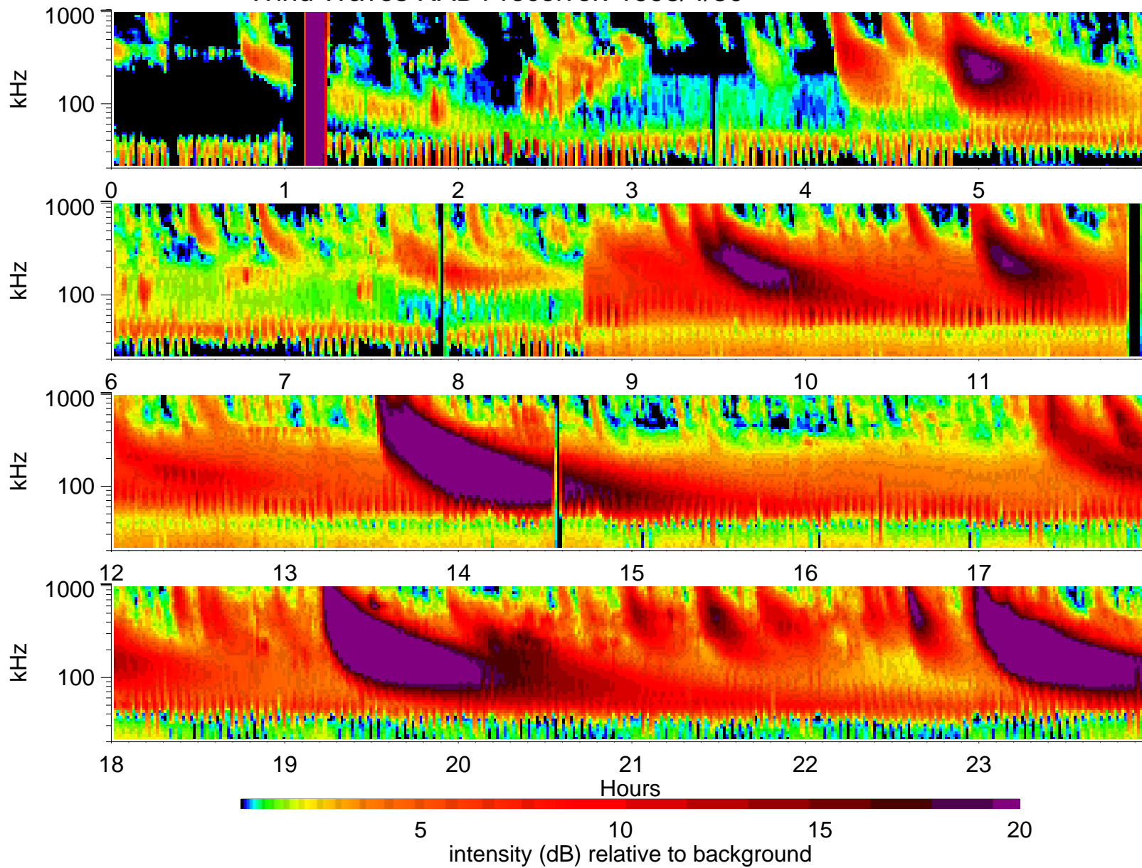
Wind Waves RAD1 receiver: 1998/4/30
