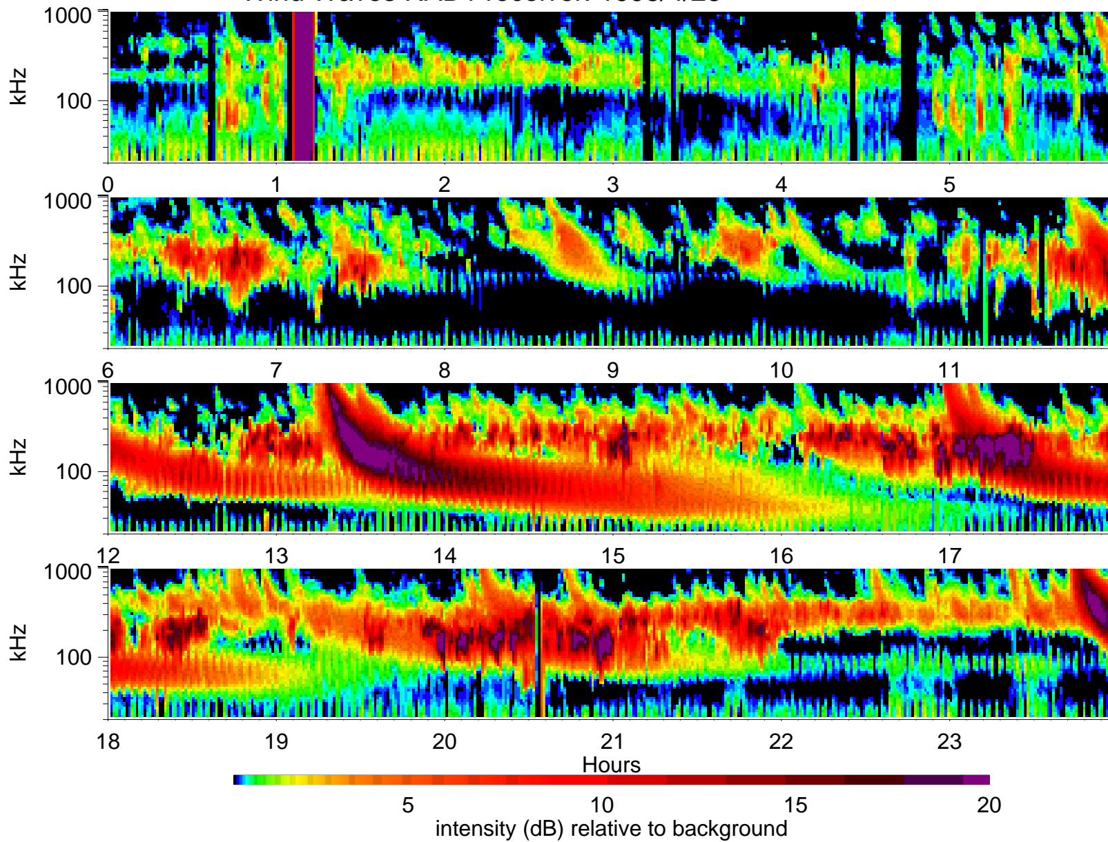
Wind Waves RAD1 receiver: 1998/4/28
