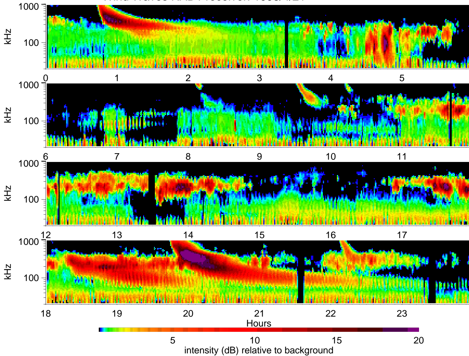
Wind Waves RAD1 receiver: 1998/4/21
