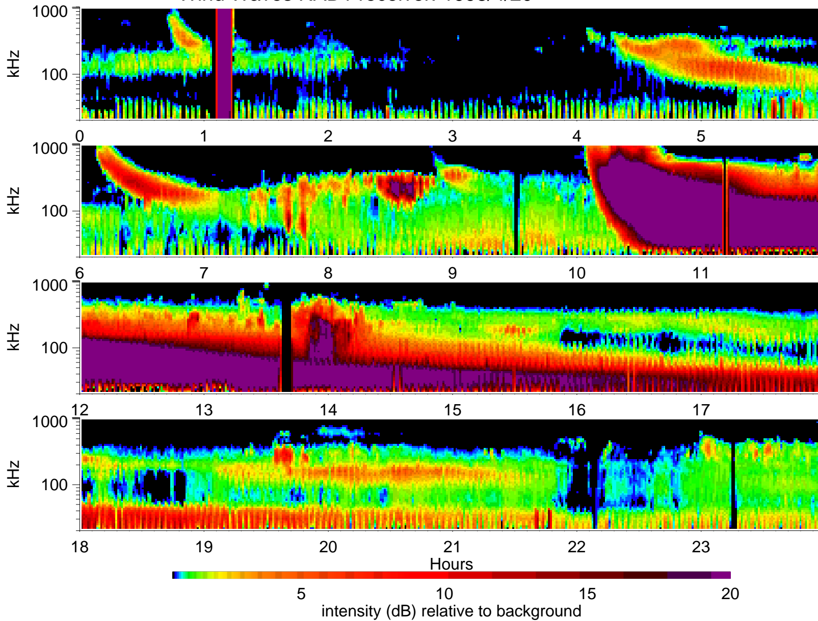
Wind Waves RAD1 receiver: 1998/4/20
