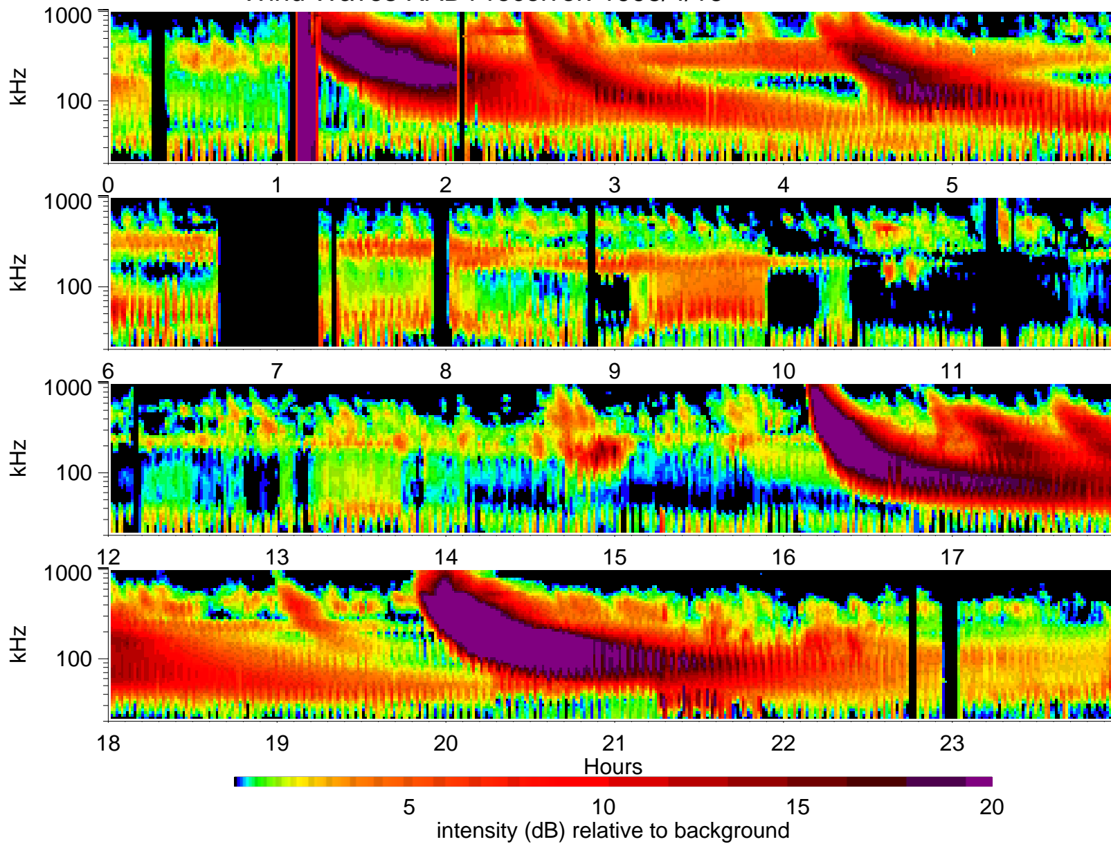
Wind Waves RAD1 receiver: 1998/4/16
