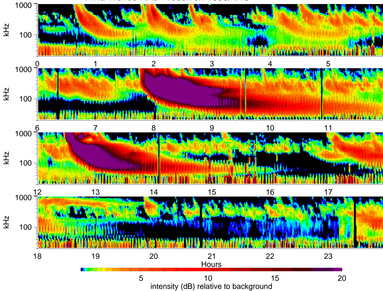
Wind Waves RAD1 receiver: 1998/4/15
