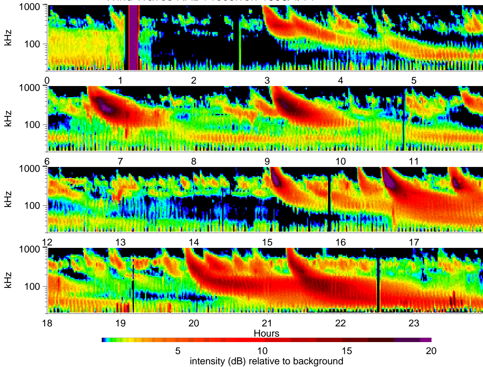
Wind Waves RAD1 receiver: 1998/4/14
