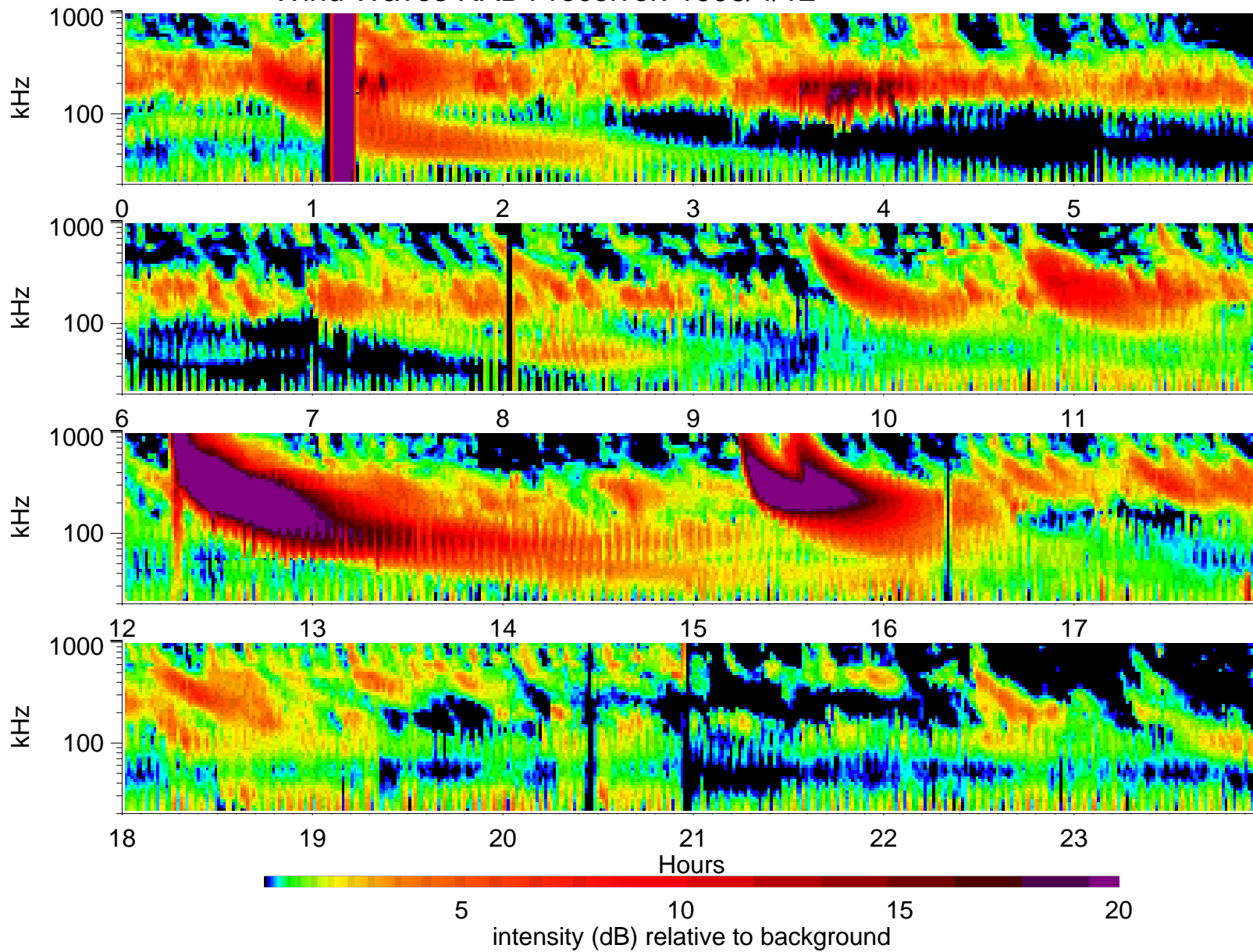
Wind Waves RAD1 receiver: 1998/4/12
