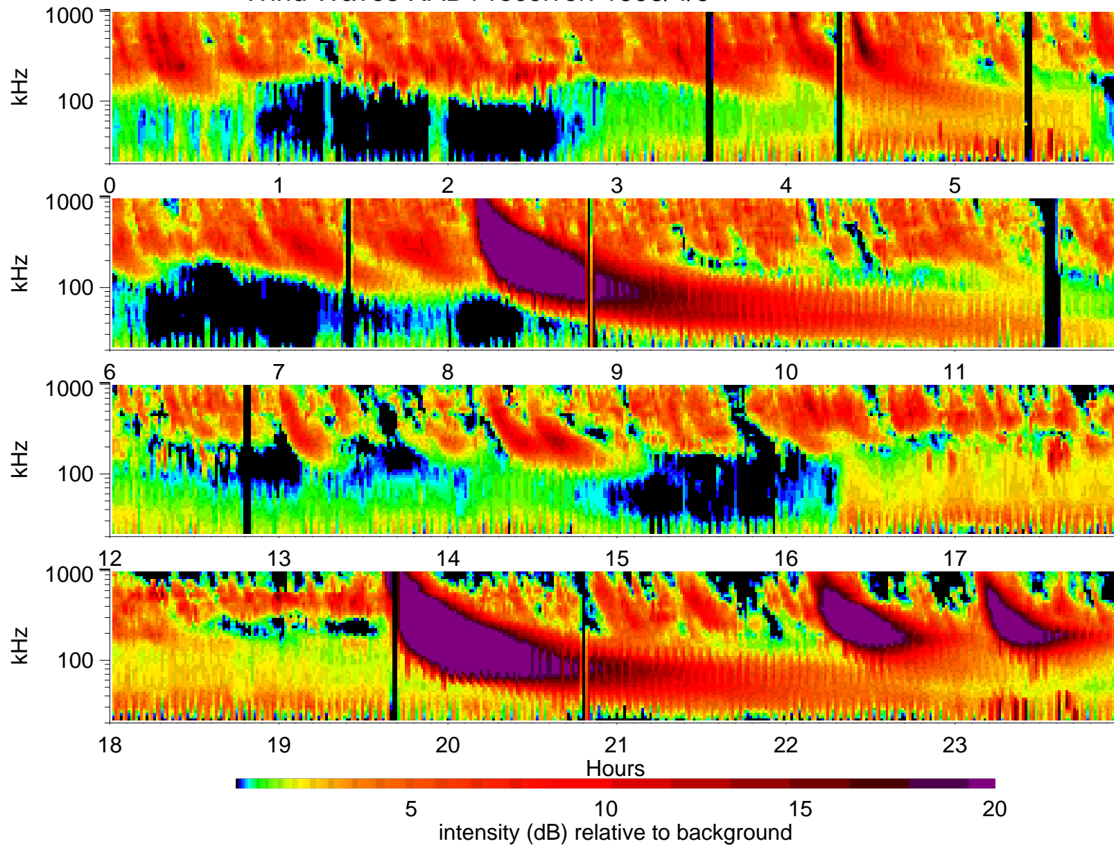
Wind Waves RAD1 receiver: 1998/4/9
