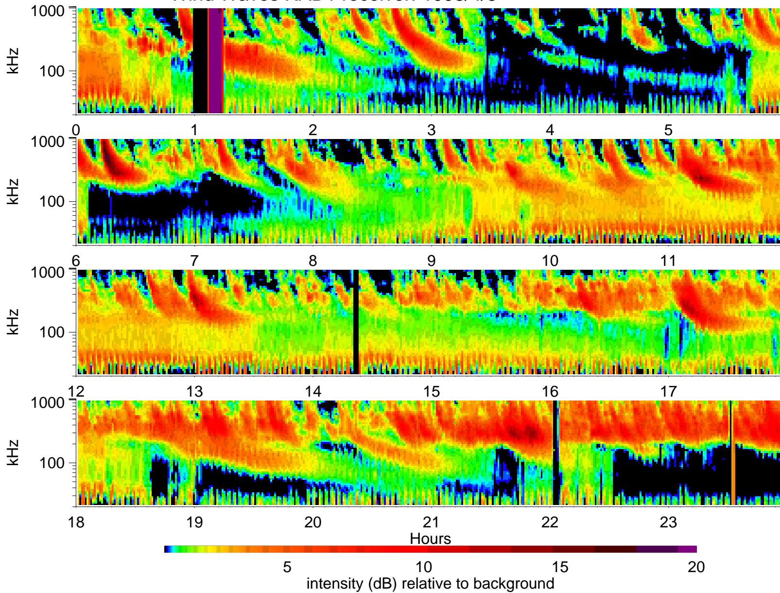
Wind Waves RAD1 receiver: 1998/4/8
