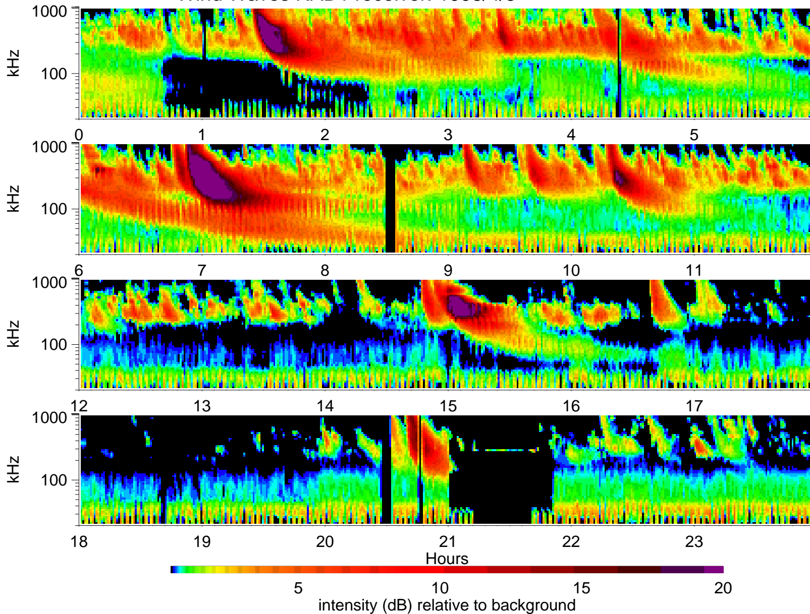
Wind Waves RAD1 receiver: 1998/4/5
