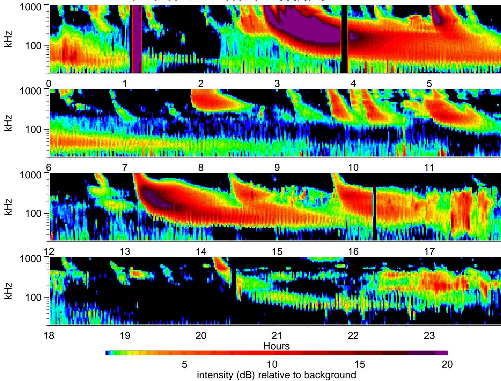
Wind Waves RAD1 receiver: 1998/3/29
