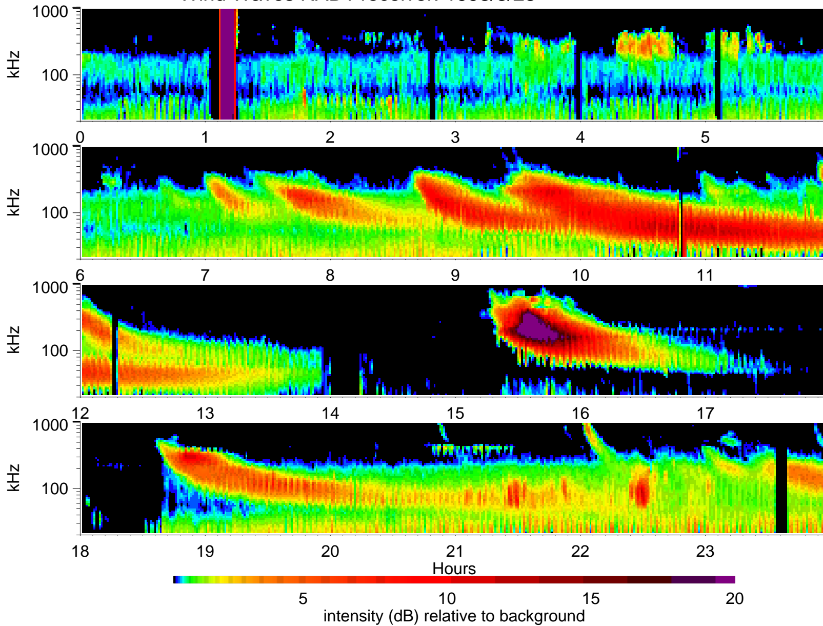
Wind Waves RAD1 receiver: 1998/3/23
