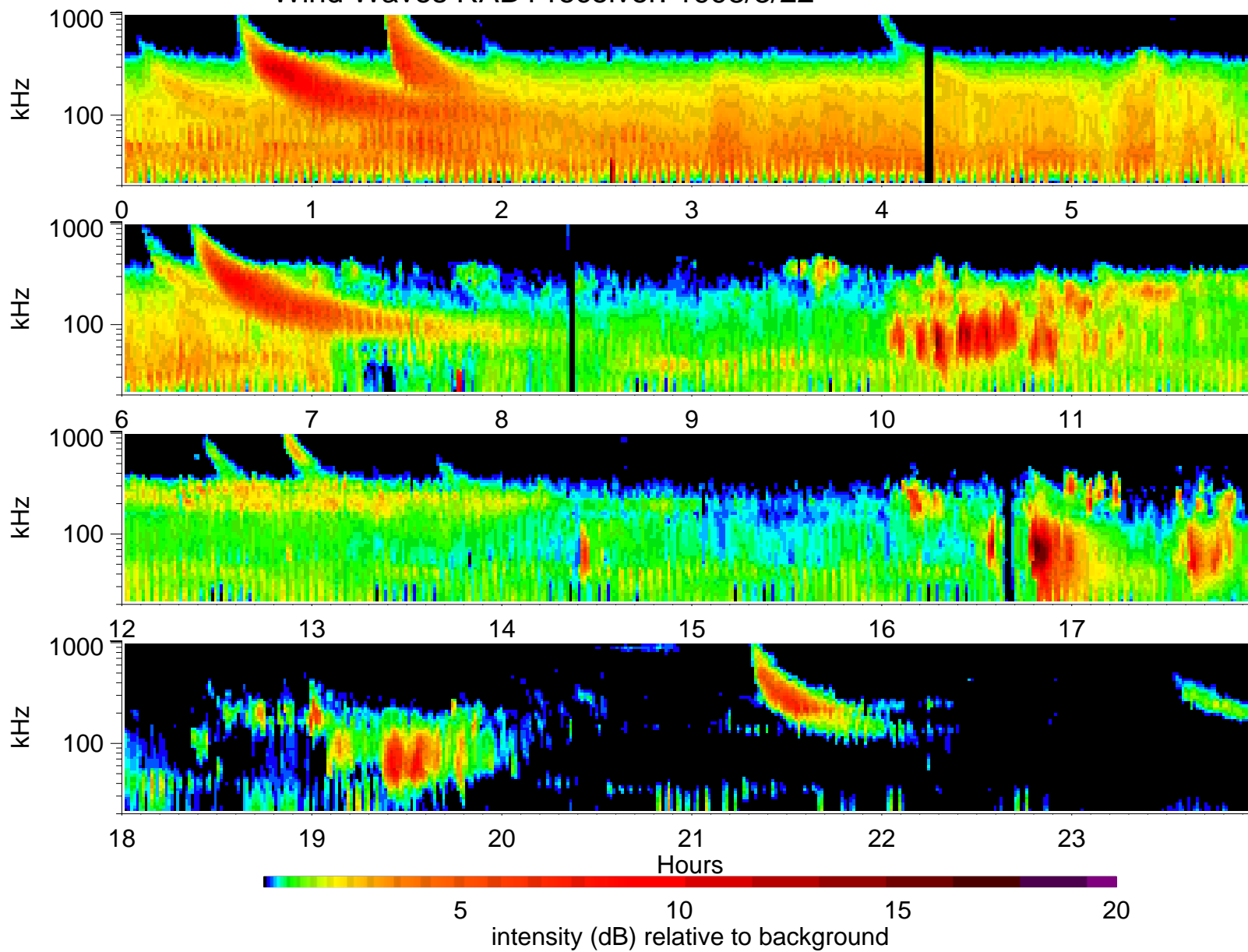
Wind Waves RAD1 receiver: 1998/3/22
